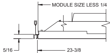
PV-LT, CURVED BLADE, PERFORATED FACE, 24" x 24"--LAY-IN PANEL
