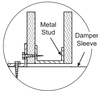
Mounting Angles
