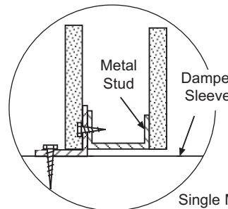
Vertical Mount (Model - VFD-10D-ISAR shown above. Optional round duct connection is a U.L. approved breakaway connection.)
