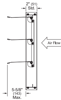
Vertical Mount
