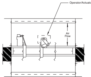
Horizontal Mount
